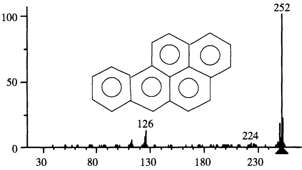
苯并[a]芘
